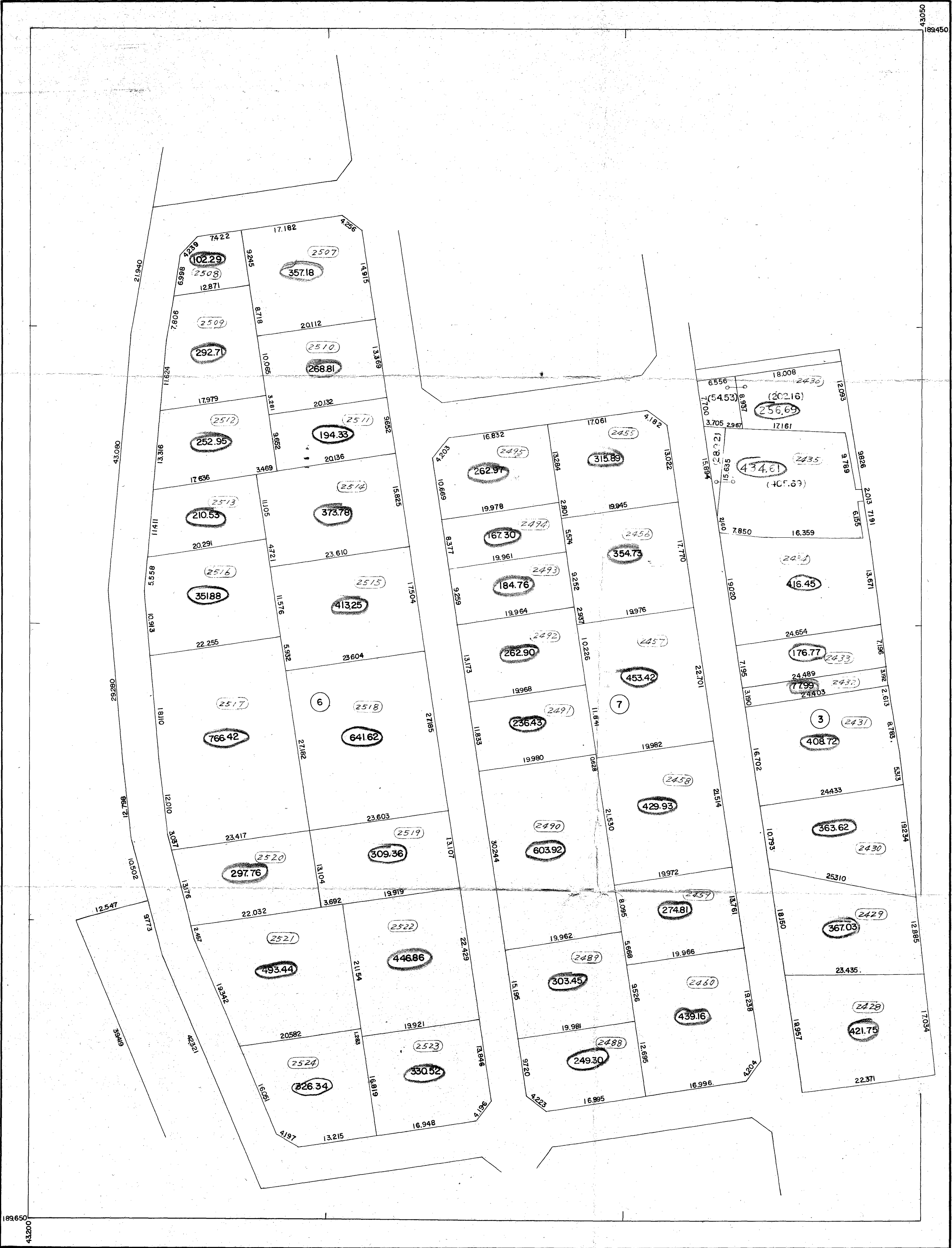
S = 1:500
